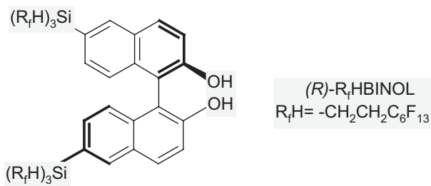
Figure 6.23. (R)\text{-}R_f\text{HBINOL} used in the asymmetric alkylation of benzaldehyde.[71]
