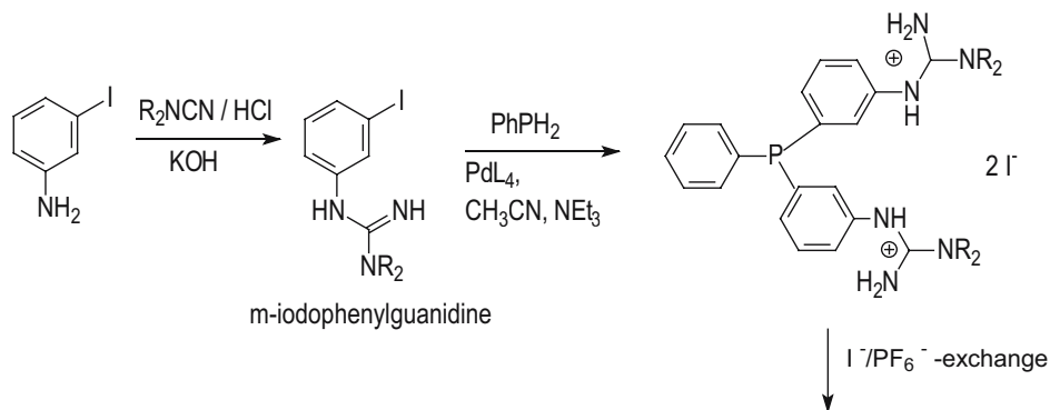
Scheme 7.4. Synthesis of a guanidinium modified triphenylphosphine ligand
