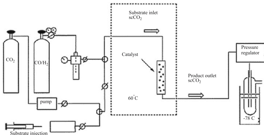
Figure 3.3. Asymmetric hydroformylation of non-volatile substrates using a stepwise injection into continuous flow reactor with \text{scCO}_2 as mobile phase
