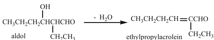
Equation 2.10. Formation of 2-ethylhex-2-enal via aldol condensation of butanal
