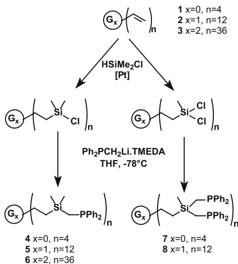
Figure 4.15. Synthesis of phosphine-functionalized carbosilane dendrimers.[31]
