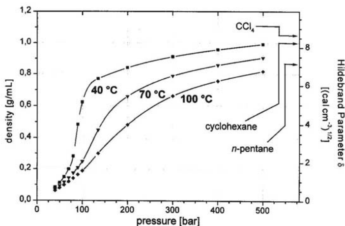
Figure 8.3. Variation of density and \delta with temperature and pressure for CO 2 . The \delta values for three typical non-polar organic solvents are also indicated (reproduced with permission from reference [1])
