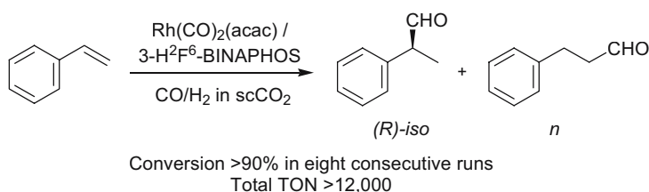
Scheme 8.3. Hydroformylation of styrene with the CO 2 -philic in situ catalyst 3-H 2 F 6 -BINAPHOS/[Rh(acac)(CO) 2 ] (2:1) using a batch-wise CESS procedure
