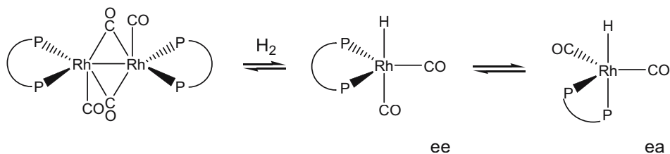
Scheme 7.8. Equilibria between different rhodium species present during hydroformylation in an ionic liquid
